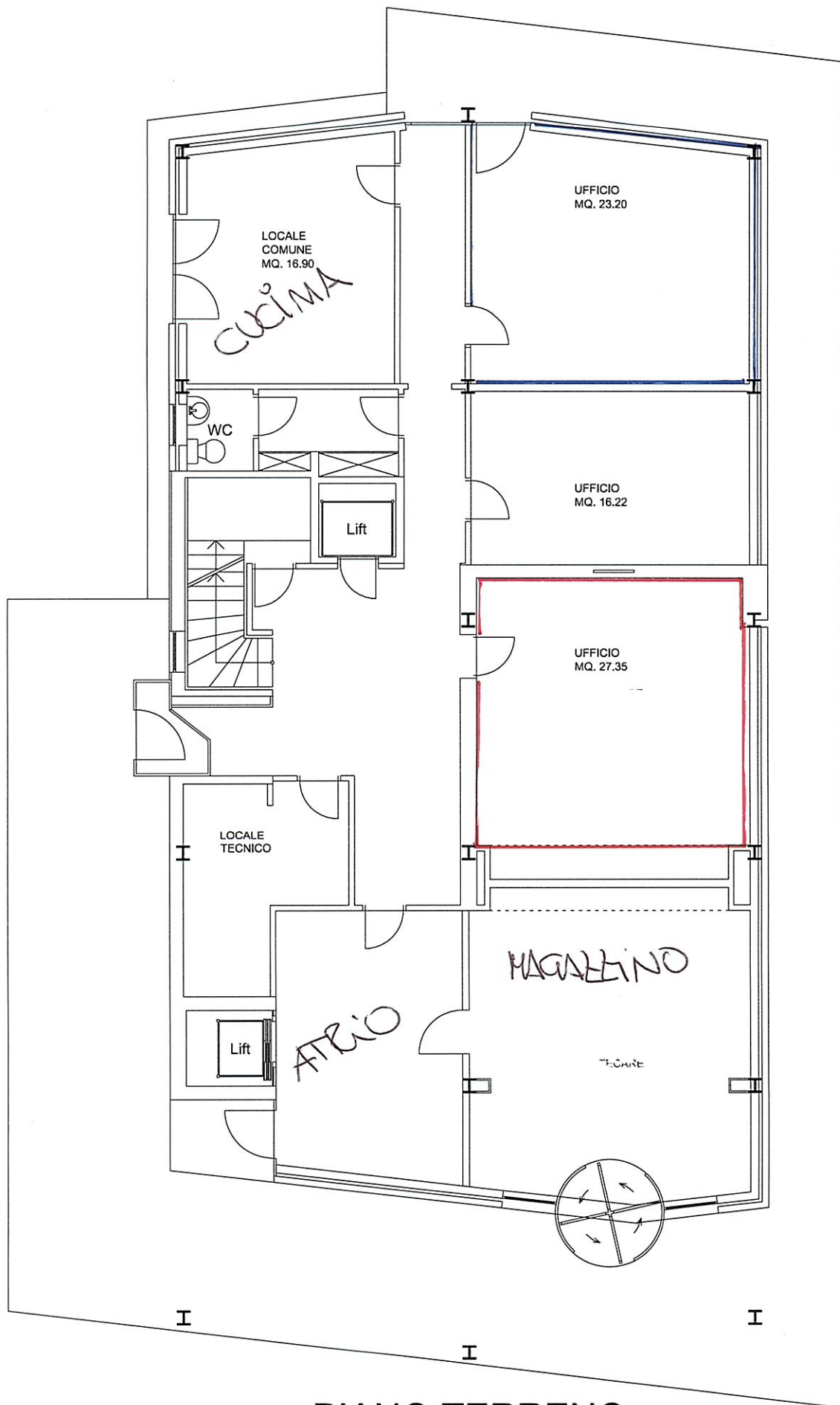
PIANO TERRENO
